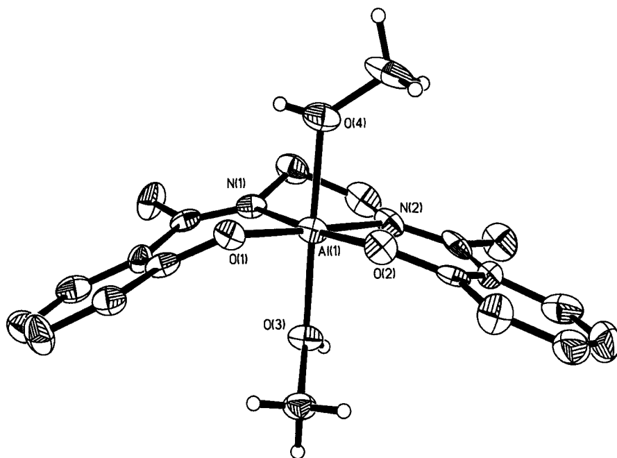
Fig. 4. The cation of [AcenAl(\text{MeOH})_2]^+ [BPh_4]^-
