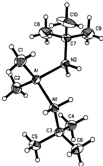
Fig. 2. The cation of [Me 2 Al(NH 2 t Bu) 2 ] + Br −
