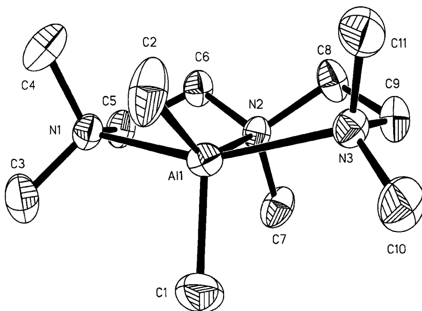
Fig. 1. The cation of [\text{Me}_2\text{Al}(\text{pmedta})]^+ [\text{Me}_2\text{AlCl}_2]^-
