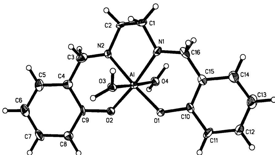
Fig. 3. The cation of [SalenAl(H 2 O) 2 ] + Cl −
