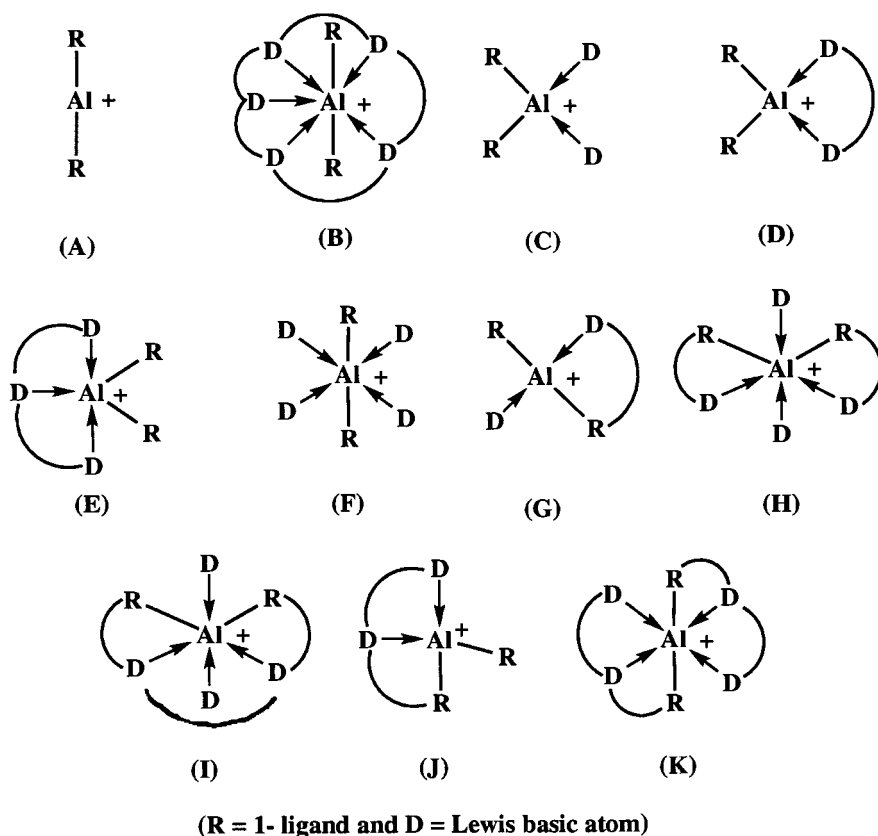
Fig. 6. General classification of group 13 cations.
